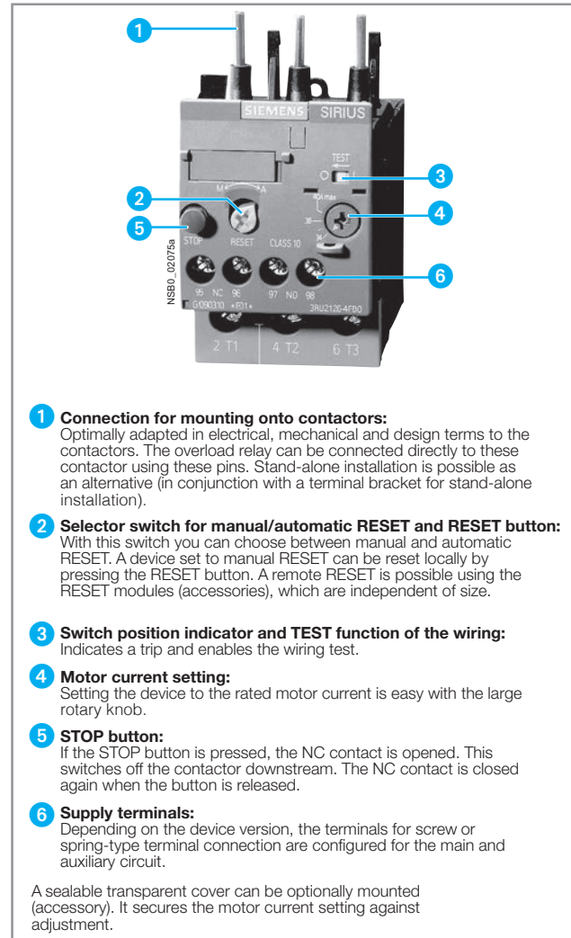
3RU21 26-4FB00 thermal overload relays
