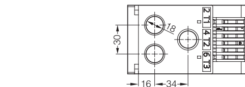
3RB30 46, 3RB31 43, size S3 with straight-through transformer
